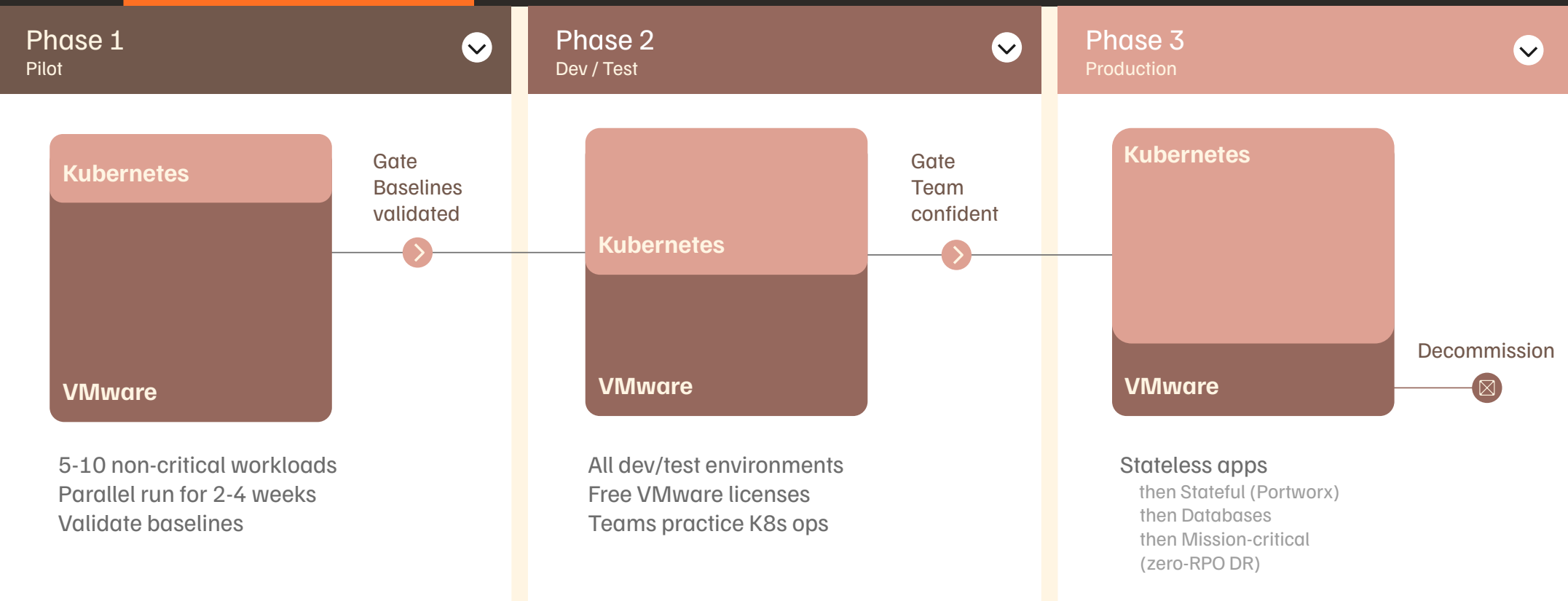
Figure 3: Three-phase migration timeline showing VMware footprint shrinking as Kubernetes adoption grows.
