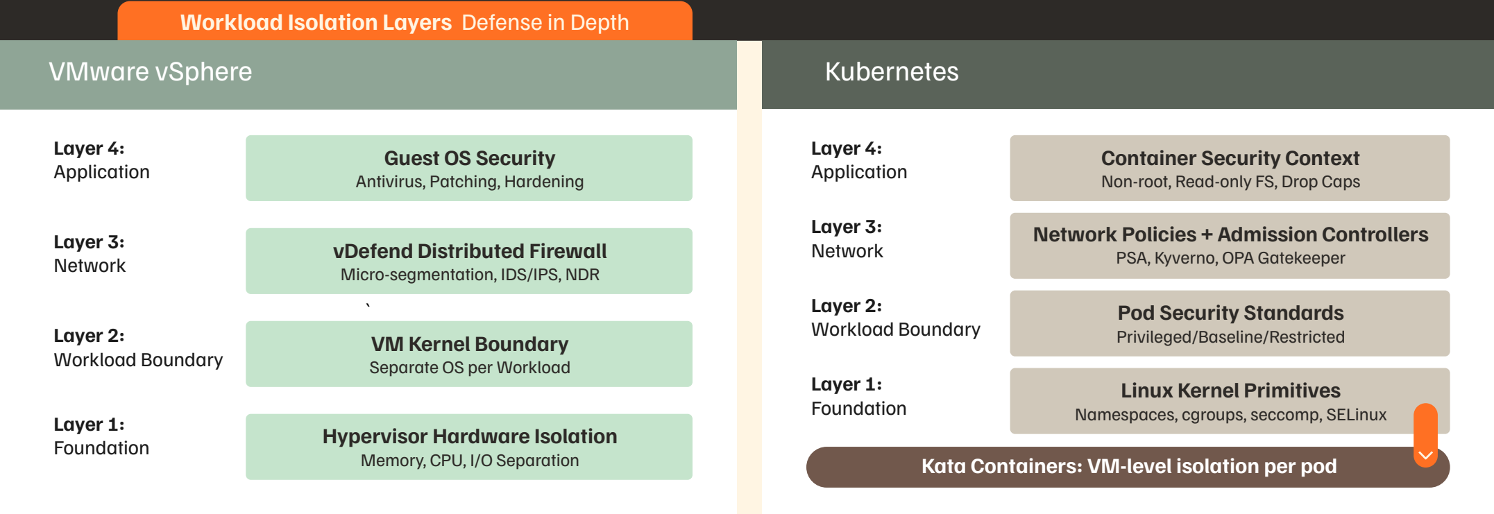
Figure 2: Defense-in-depth with VMware vs Kubernetes
